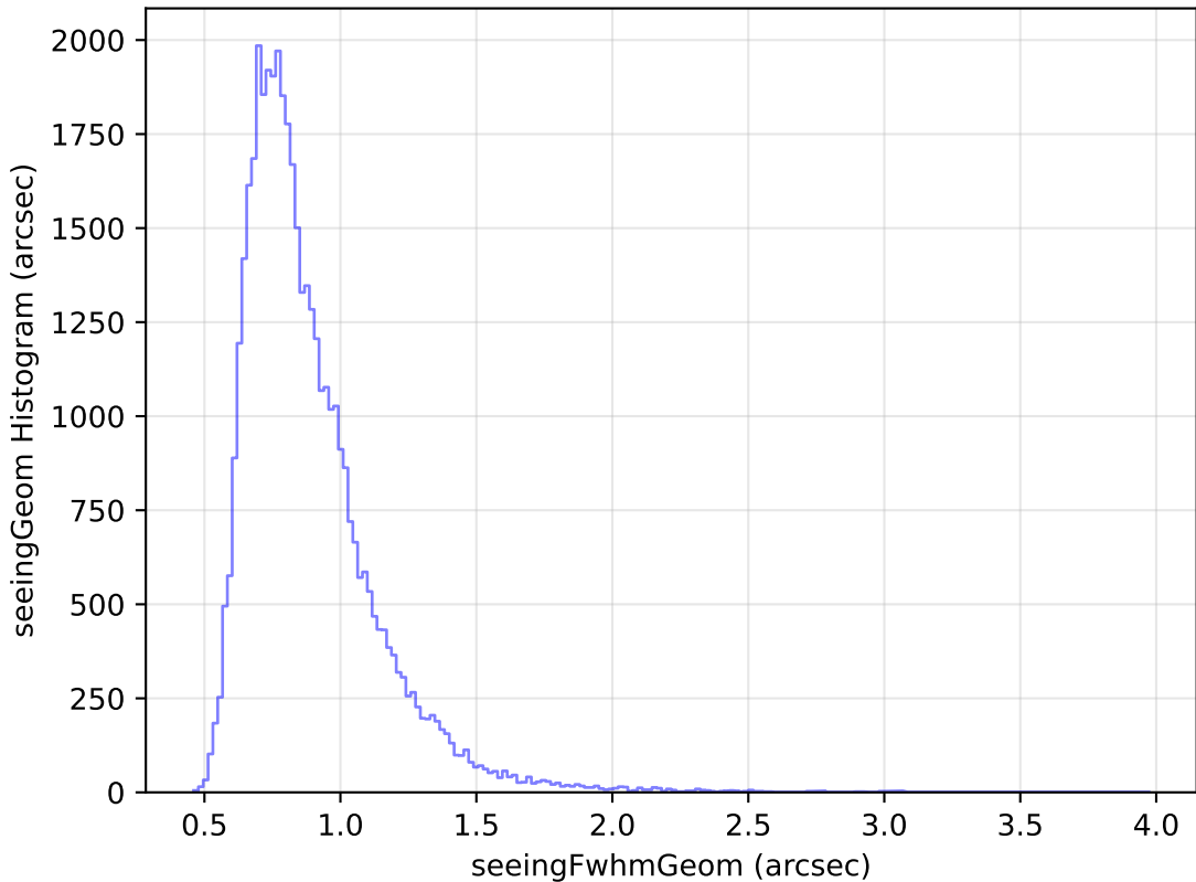
too_elab_r64_d3_griz_v3.4_10yrs Yr 1 z band: seeingGeom Histogram
