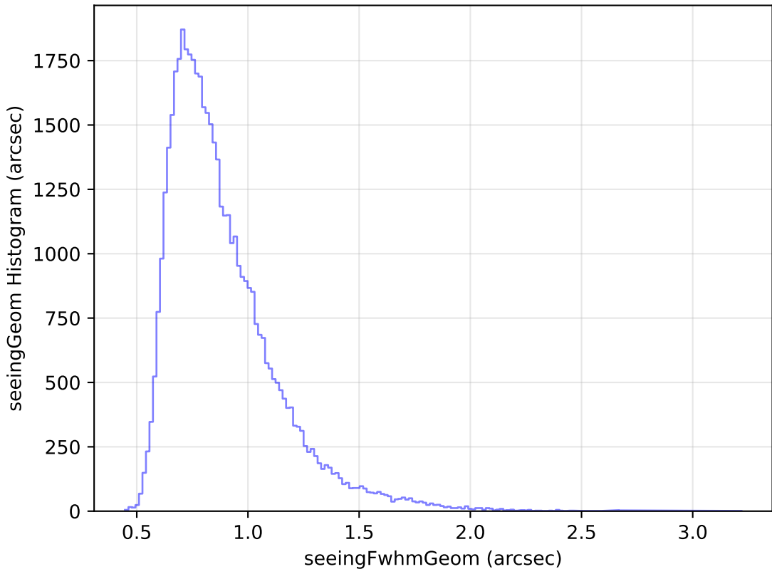
too_elab_r64_d3_griz_v3.4_10yrs Yr 1 r band: seeingGeom Histogram
