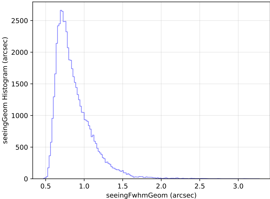
too_elab_r64_d3_griz_v3.4_10yrs Yr 1 i band: seeingGeom Histogram
