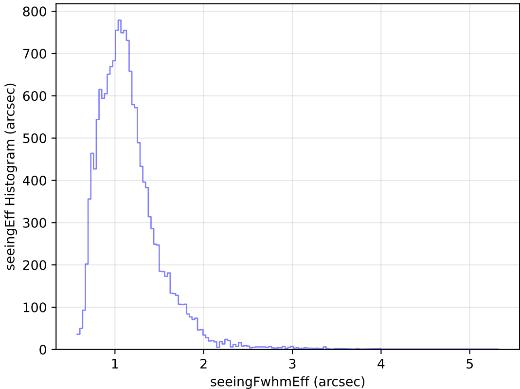
too_elab_r64_d3_griz_v3.4_10yrs Yr 1 u band: seeingEff Histogram
