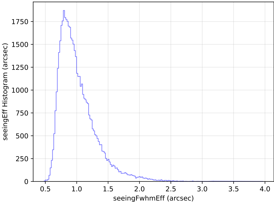
too_elab_r64_d3_griz_v3.4_10yrs Yr 1 r band: seeingEff Histogram
