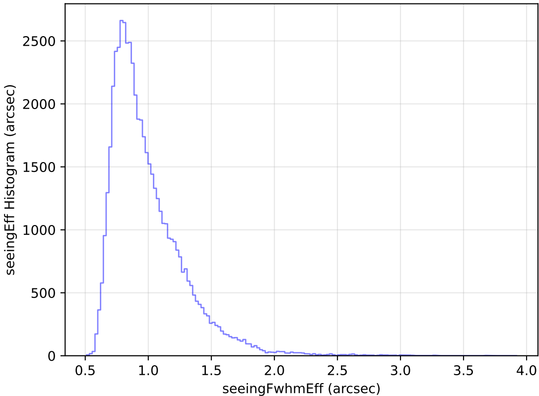
too_elab_r64_d3_griz_v3.4_10yrs Yr 1 i band: seeingEff Histogram
