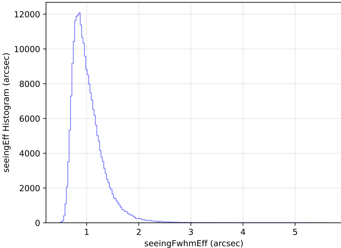
too_elab_r64_d3_griz_v3.4_10yrs Yr 1 all bands: seeingEff Histogram
