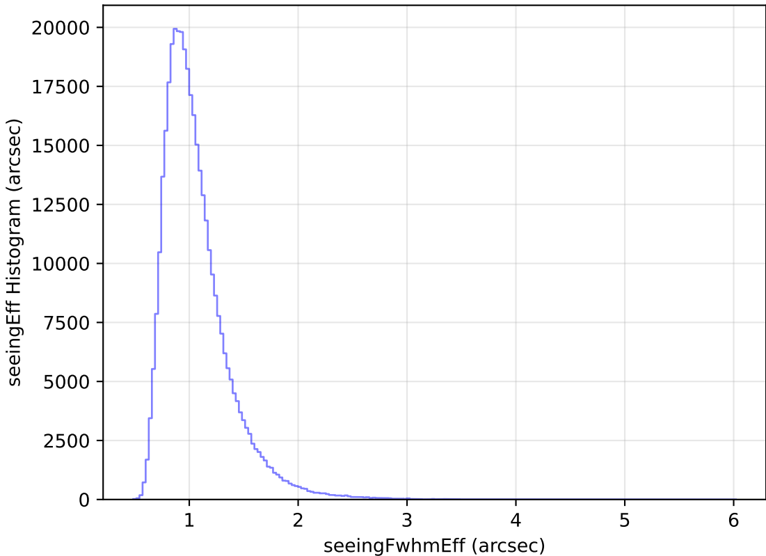
too_elab_r64_d3_griz_v3.4_10yrs WFD y band: seeingEff Histogram
