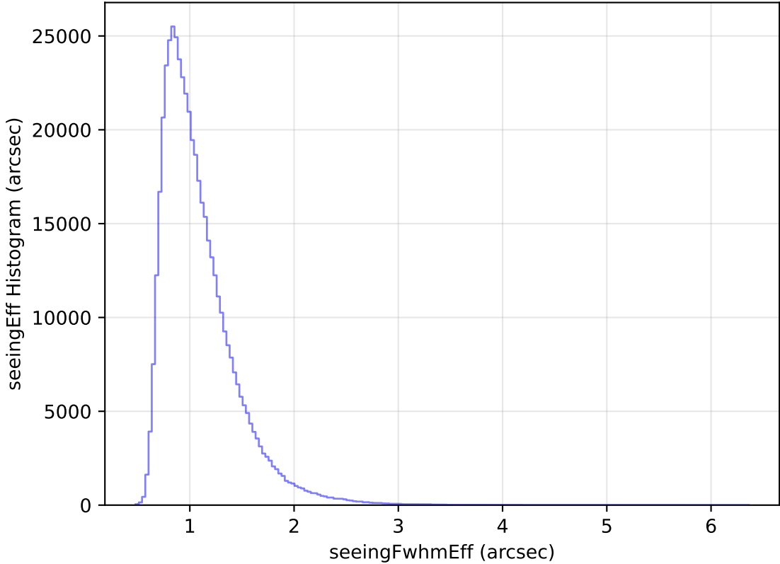
too_elab_r64_d3_griz_v3.4_10yrs WFD i band: seeingEff Histogram
