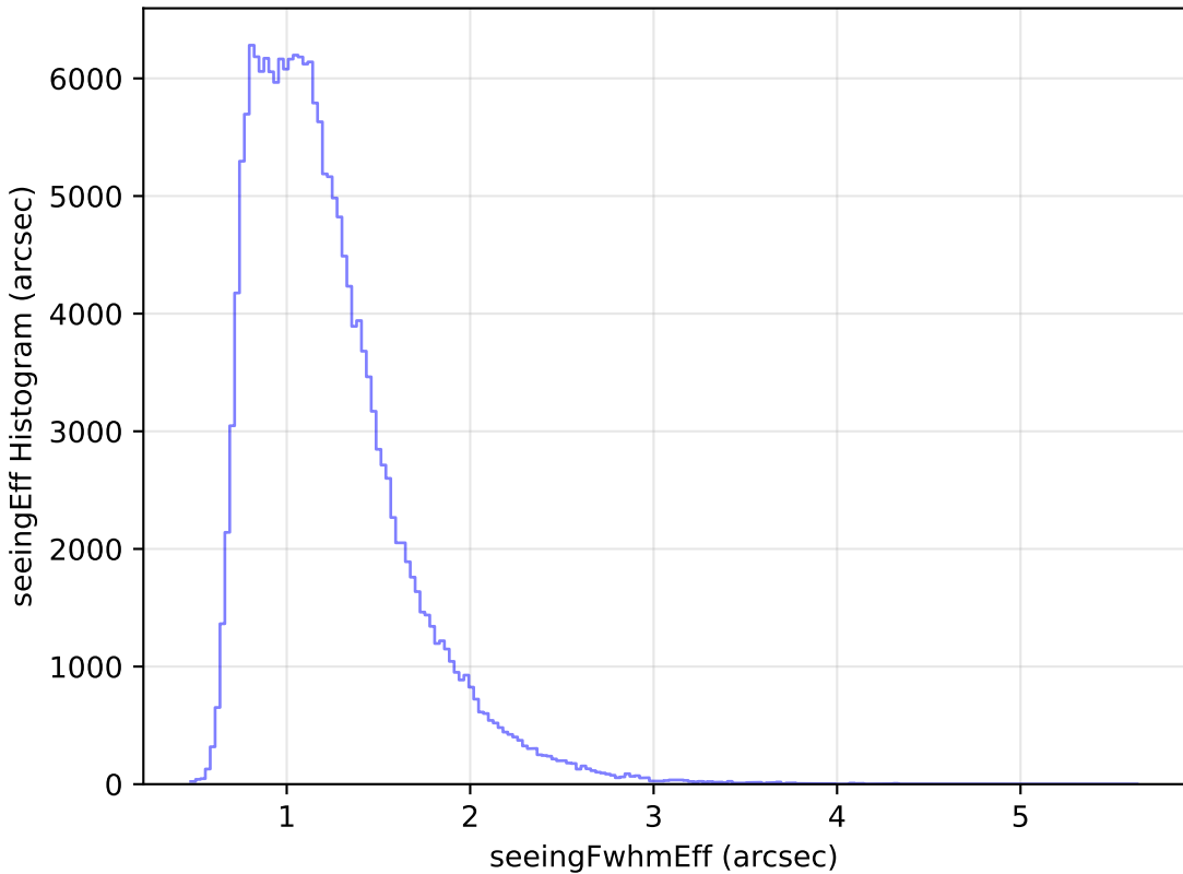
too_elab_r64_d3_griz_v3.4_10yrs WFD g band: seeingEff Histogram
