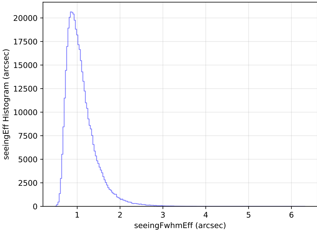
too_elab_r64_d3_griz_v3.4_10yrs All sky z band: seeingEff Histogram
