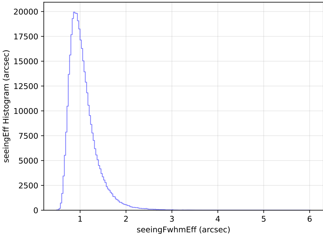
too_elab_r64_d3_griz_v3.4_10yrs All sky y band: seeingEff Histogram
