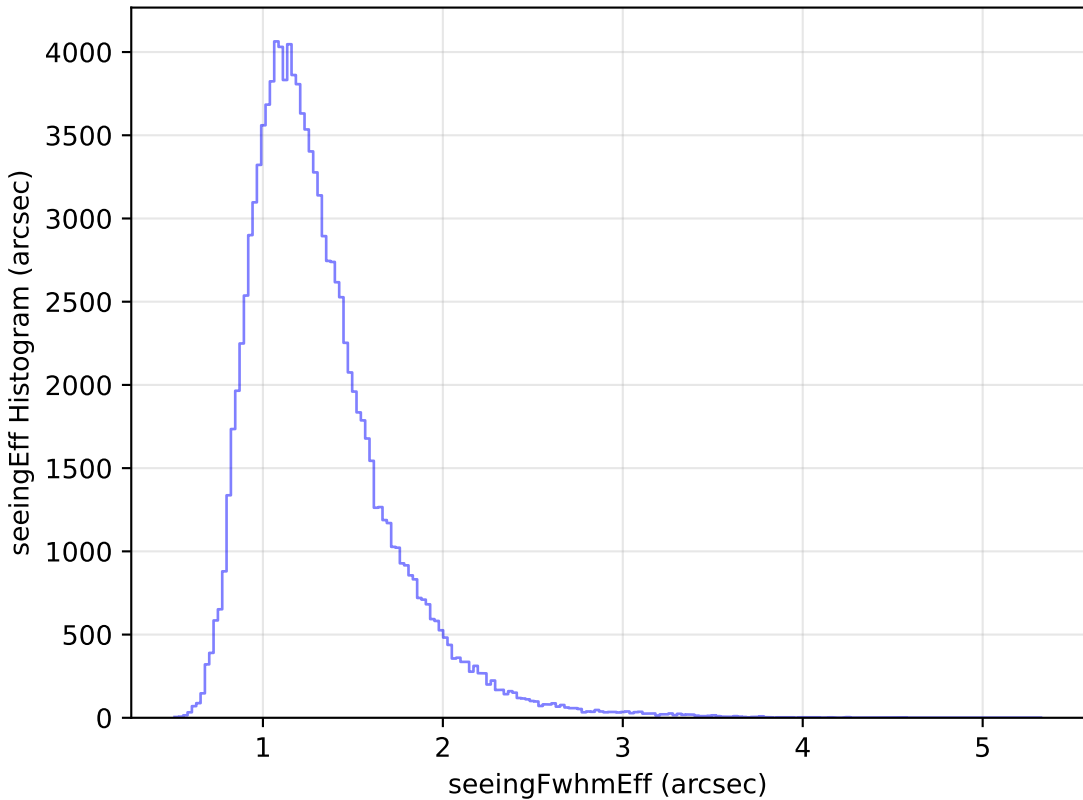
too_elab_r64_d3_griz_v3.4_10yrs All sky u band: seeingEff Histogram
