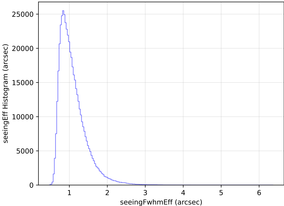
too_elab_r64_d3_griz_v3.4_10yrs All sky i band: seeingEff Histogram
