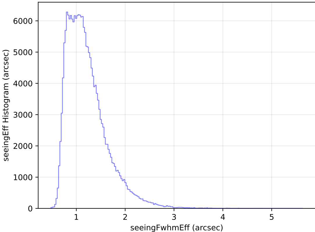
too_elab_r64_d3_griz_v3.4_10yrs All sky g band: seeingEff Histogram
