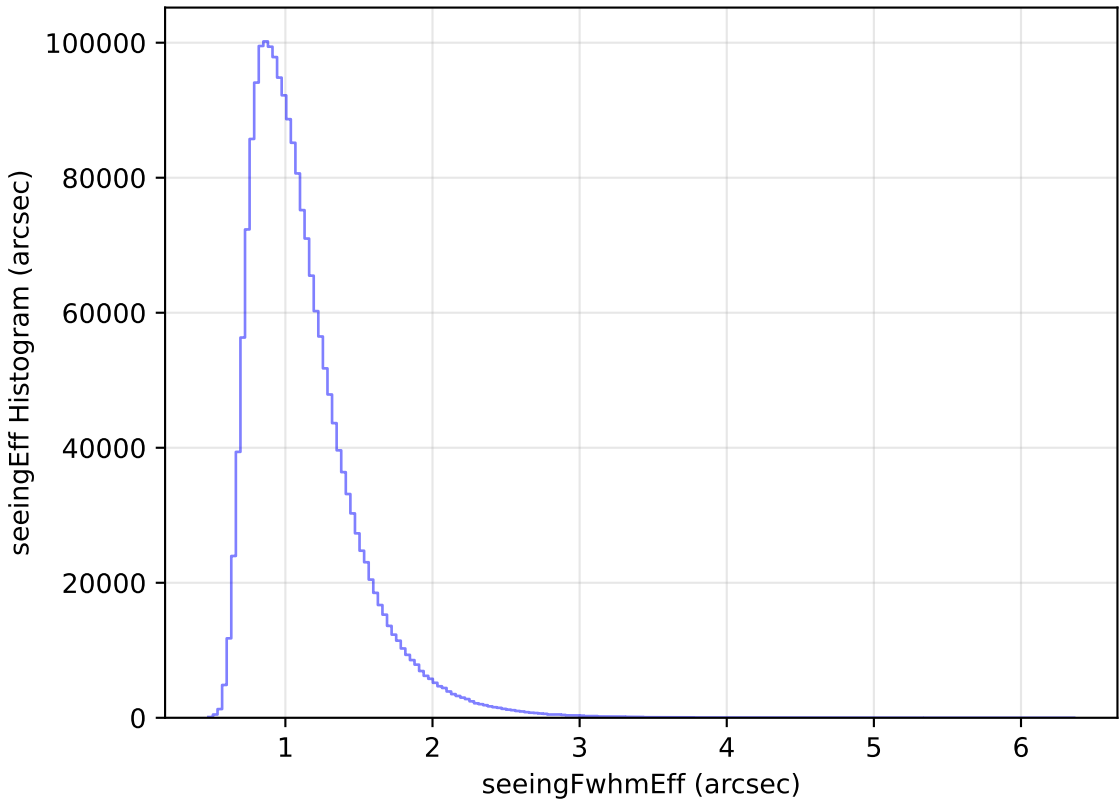
too_elab_r64_d3_griz_v3.4_10yrs All sky all bands: seeingEff Histogram
