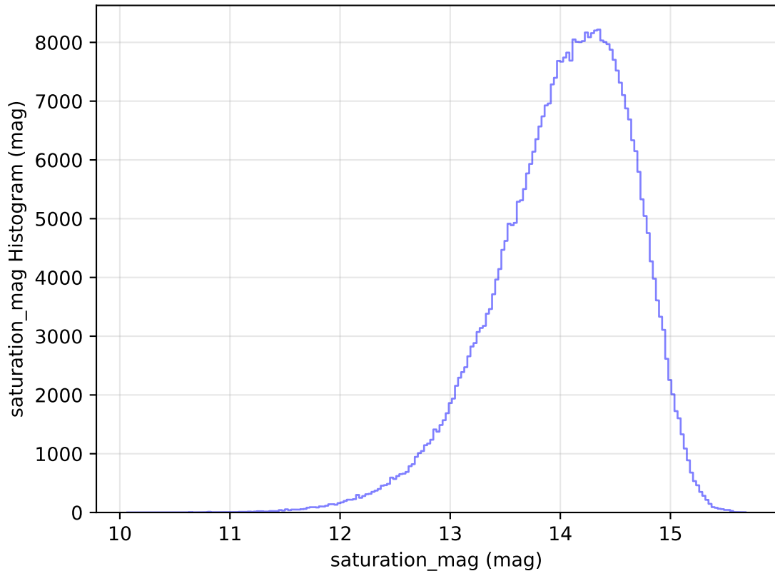
too_elab_r64_d3_griz_v3.4_10yrs WFD z band: saturation_mag Histogram
