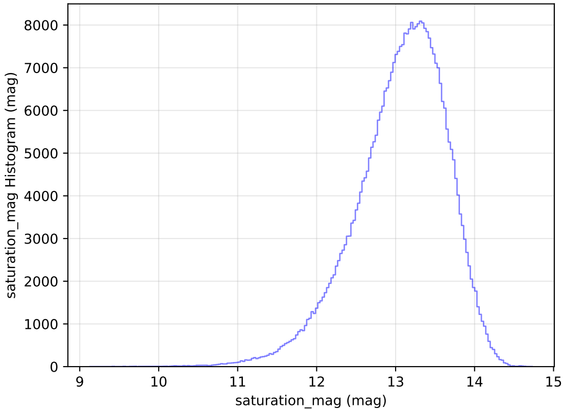
too_elab_r64_d3_griz_v3.4_10yrs WFD y band: saturation_mag Histogram
