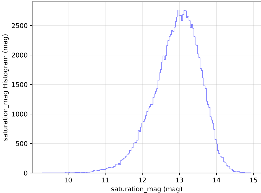
too_elab_r64_d3_griz_v3.4_10yrs WFD u band: saturation_mag Histogram
