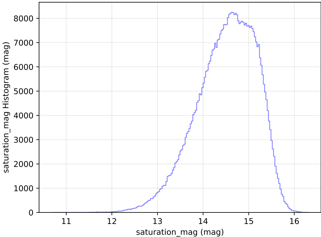
too_elab_r64_d3_griz_v3.4_10yrs WFD r band: saturation_mag Histogram
