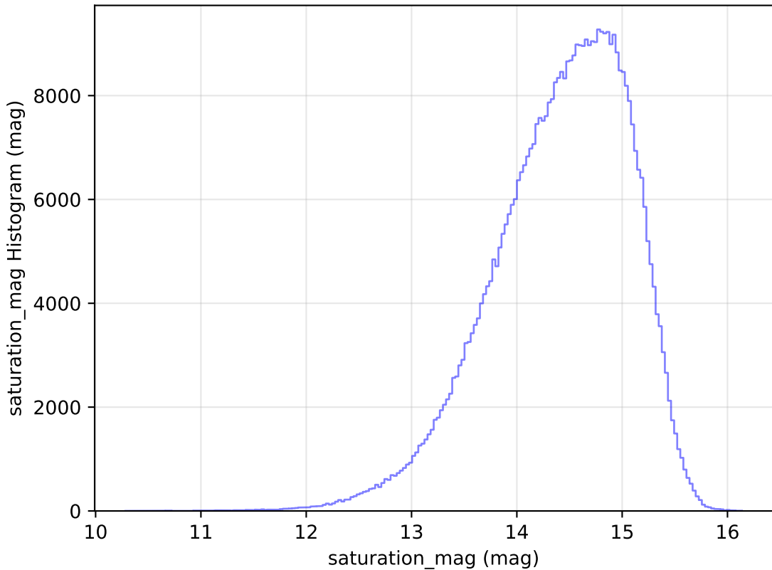
too_elab_r64_d3_griz_v3.4_10yrs WFD i band: saturation_mag Histogram
