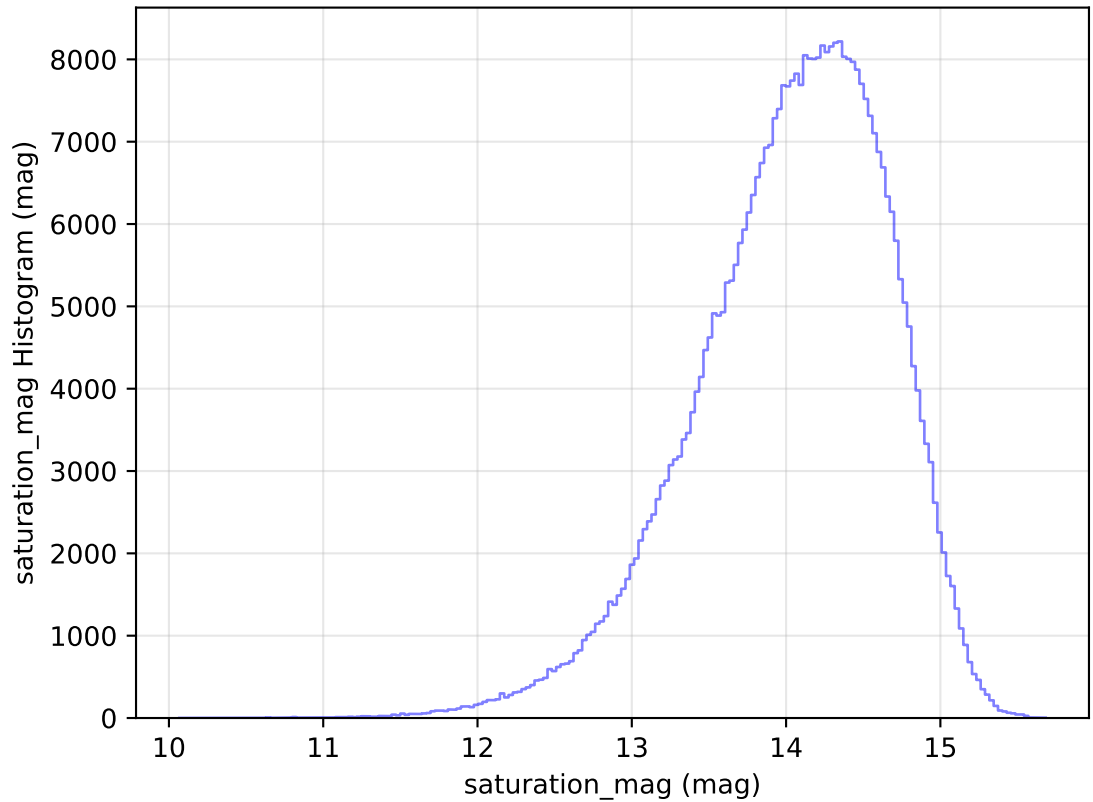
too_elab_r64_d3_griz_v3.4_10yrs All sky z band: saturation_mag Histogram
