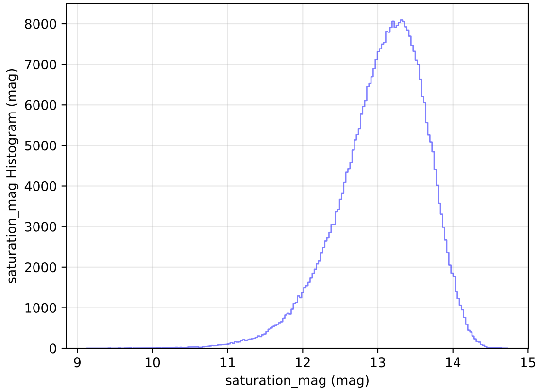
too_elab_r64_d3_griz_v3.4_10yrs All sky y band: saturation_mag Histogram
