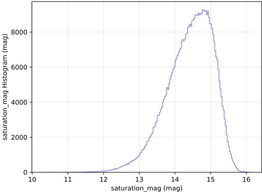
too_elab_r64_d3_griz_v3.4_10yrs All sky i band: saturation_mag Histogram
