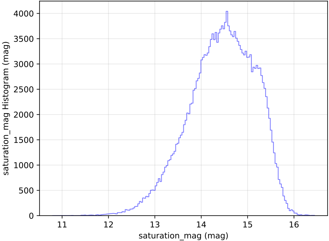
too_elab_r64_d3_griz_v3.4_10yrs All sky g band: saturation_mag Histogram
