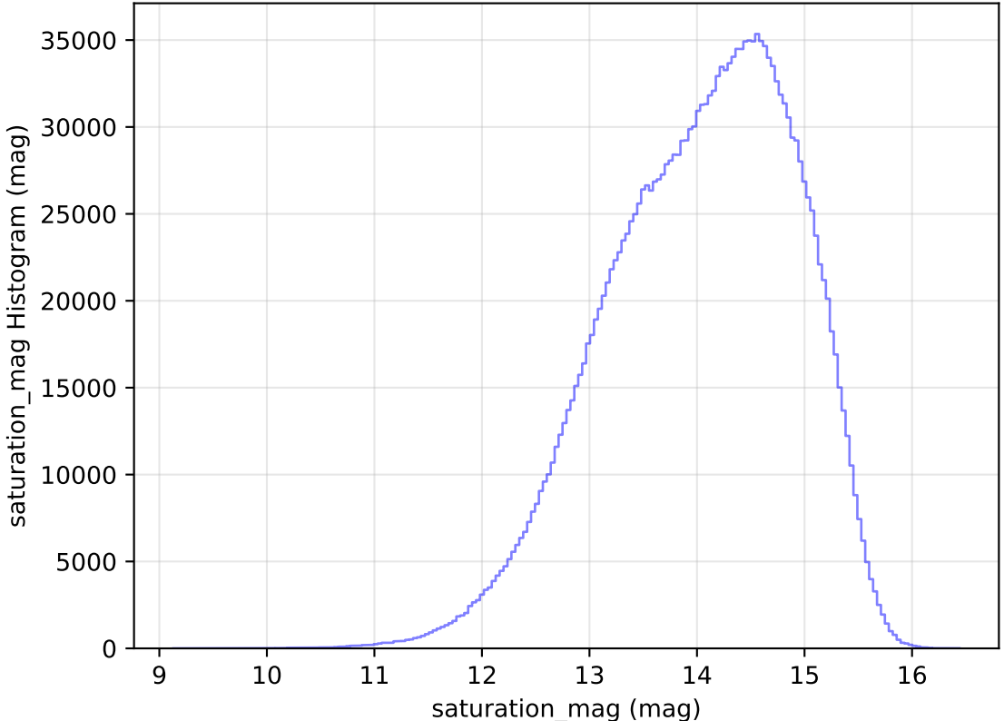
too_elab_r64_d3_griz_v3.4_10yrs All sky all bands: saturation_mag Histogram
