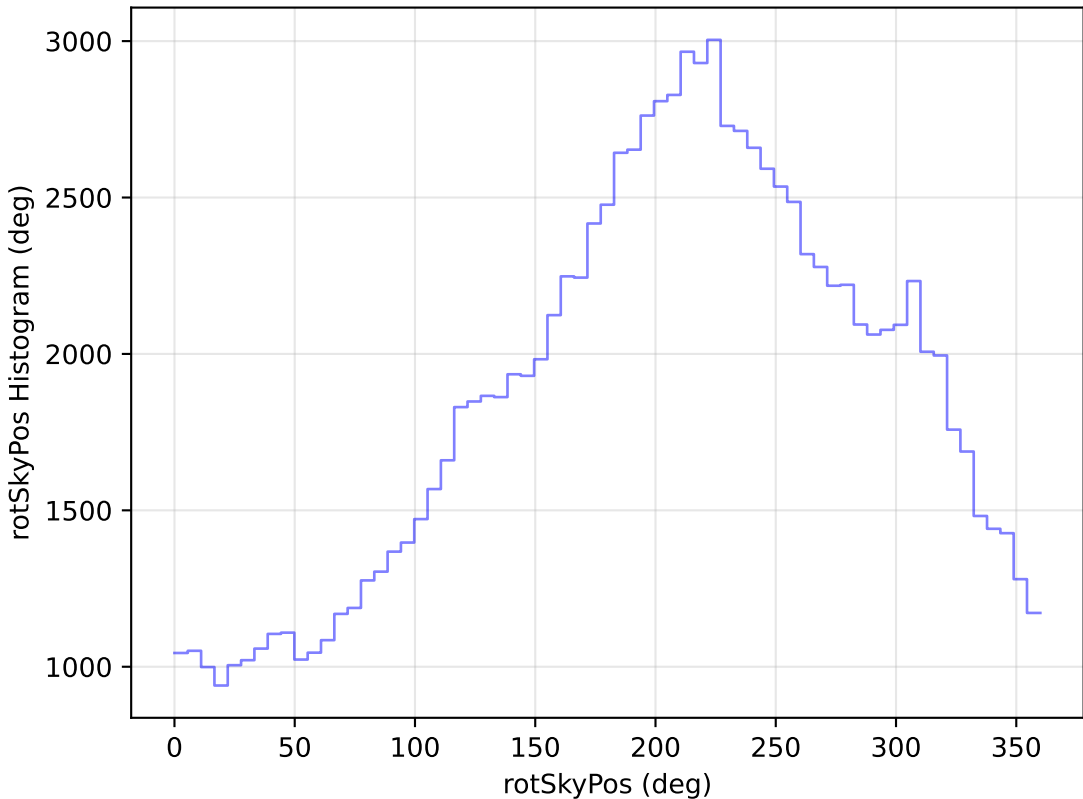
too_elab_r64_d3_griz_v3.4_10yrs WFD u band: rotSkyPos Histogram
