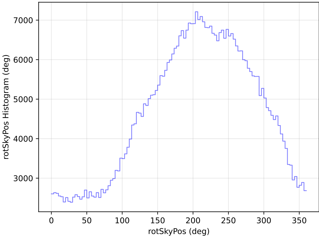
too_elab_r64_d3_griz_v3.4_10yrs WFD i band: rotSkyPos Histogram
