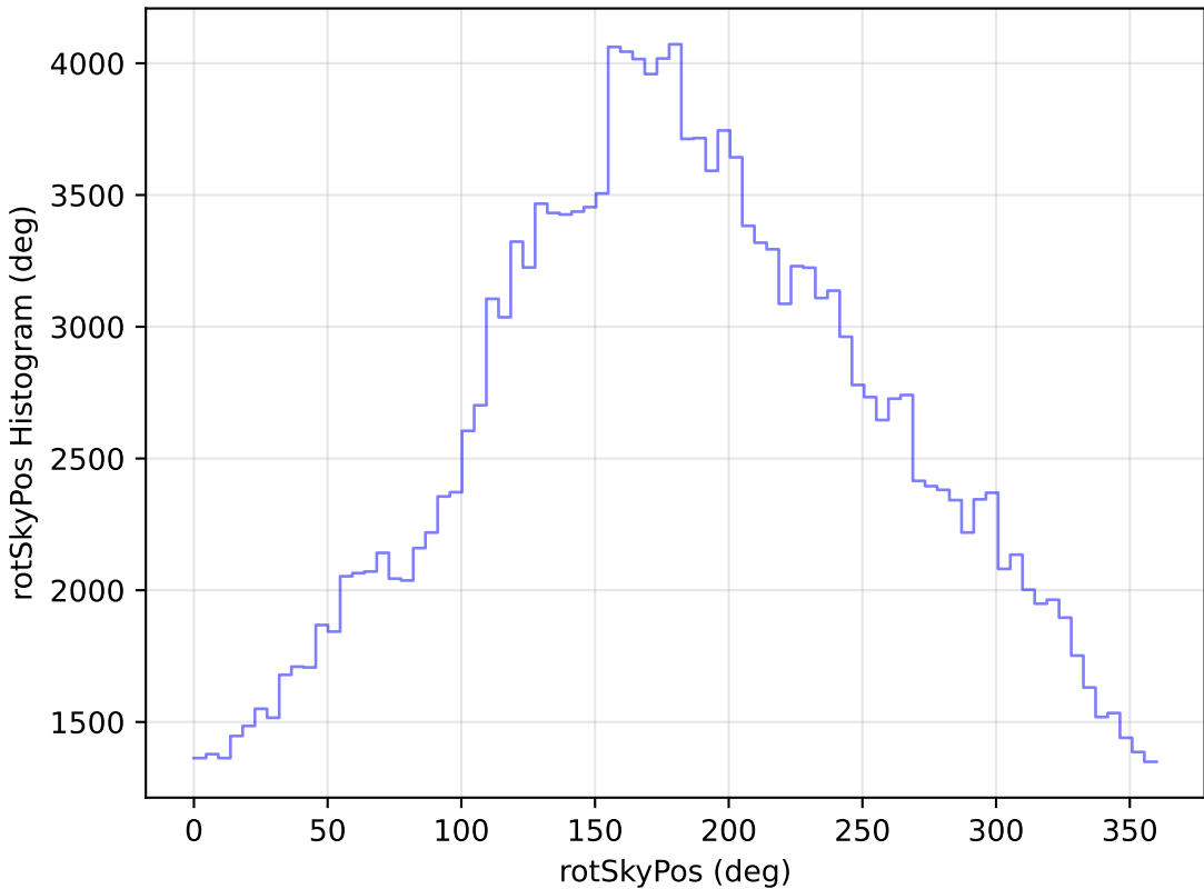
too_elab_r64_d3_griz_v3.4_10yrs WFD g band: rotSkyPos Histogram
