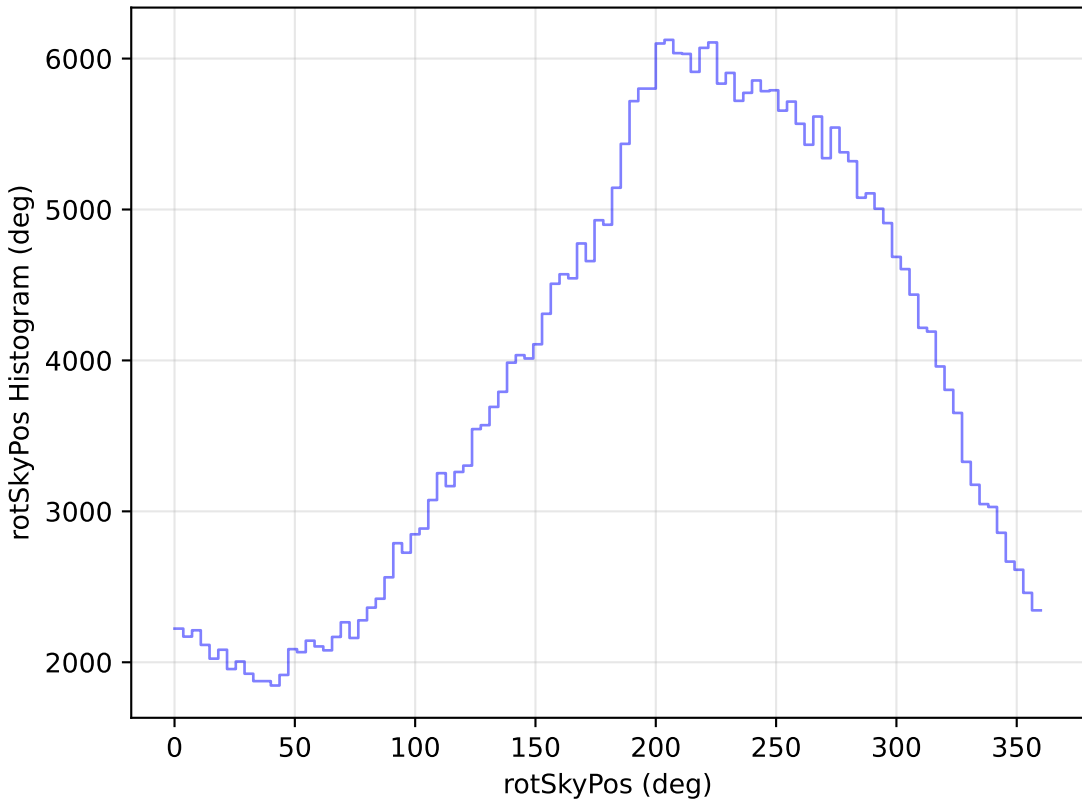
too_elab_r64_d3_griz_v3.4_10yrs All sky y band: rotSkyPos Histogram
