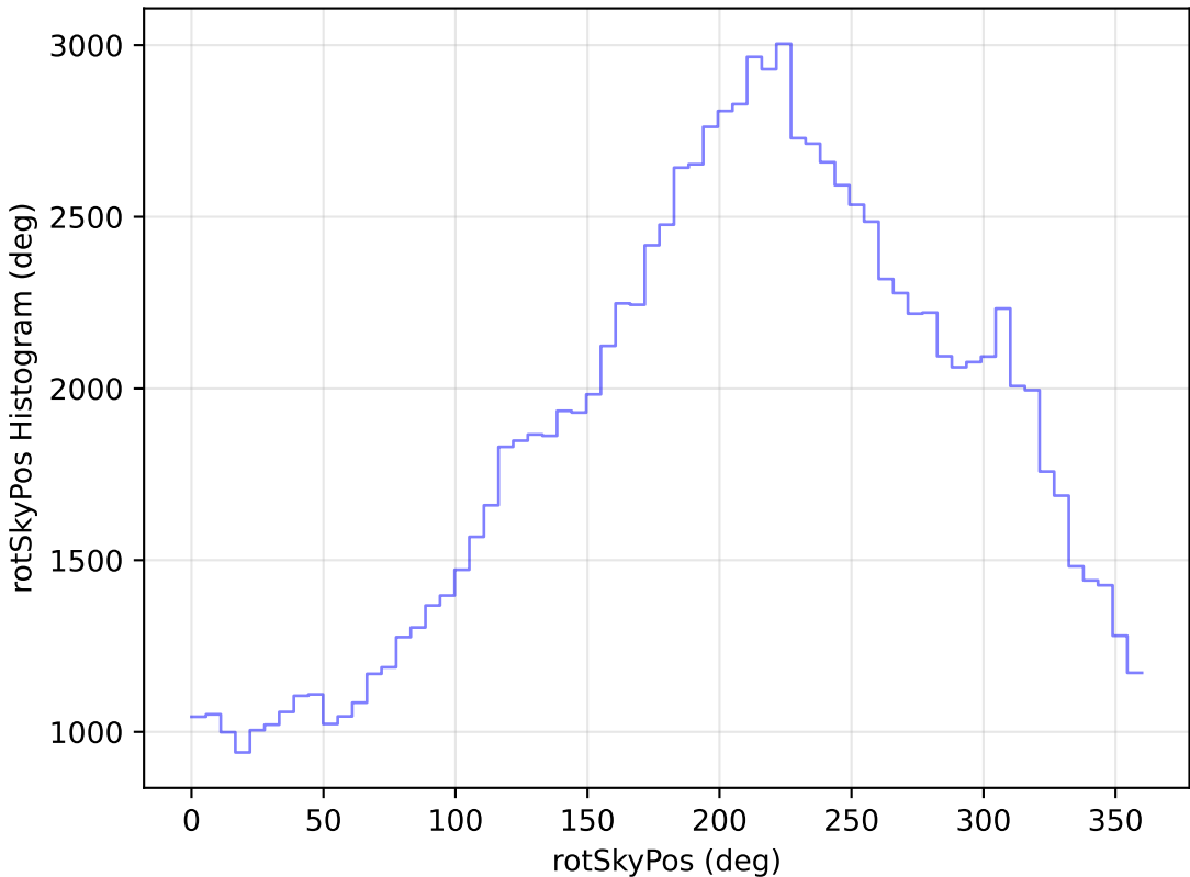
too_elab_r64_d3_griz_v3.4_10yrs All sky u band: rotSkyPos Histogram
