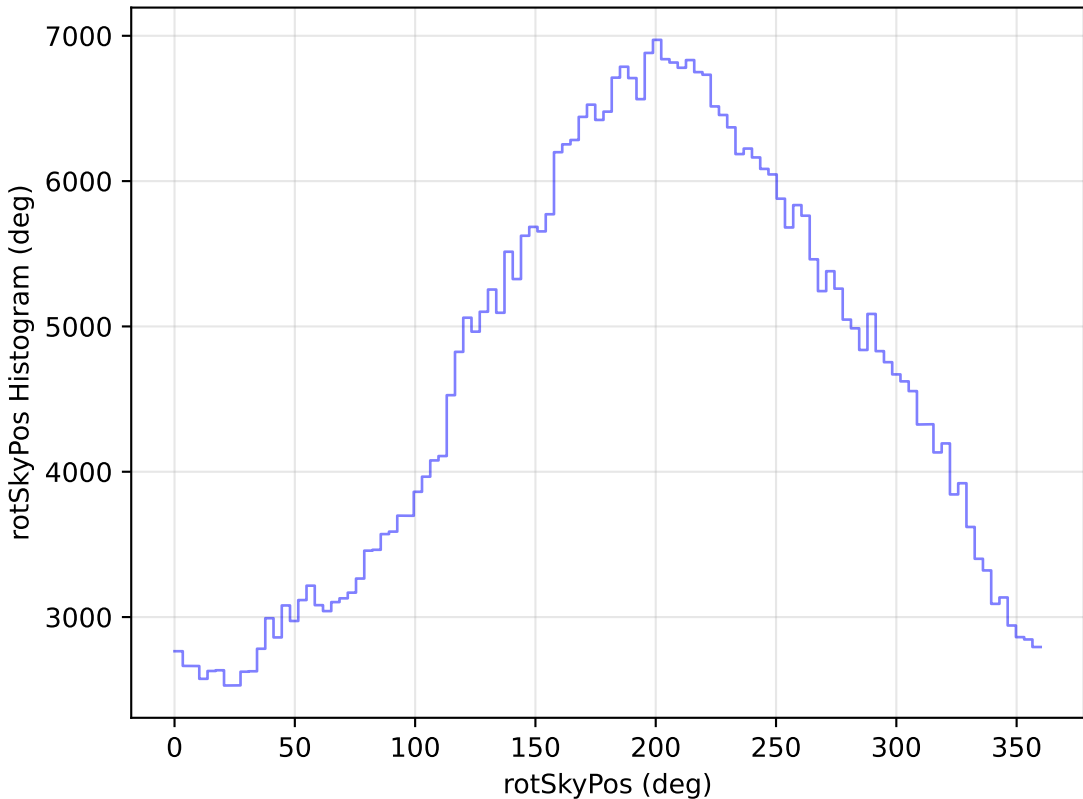
too_elab_r64_d3_griz_v3.4_10yrs All sky r band: rotSkyPos Histogram
