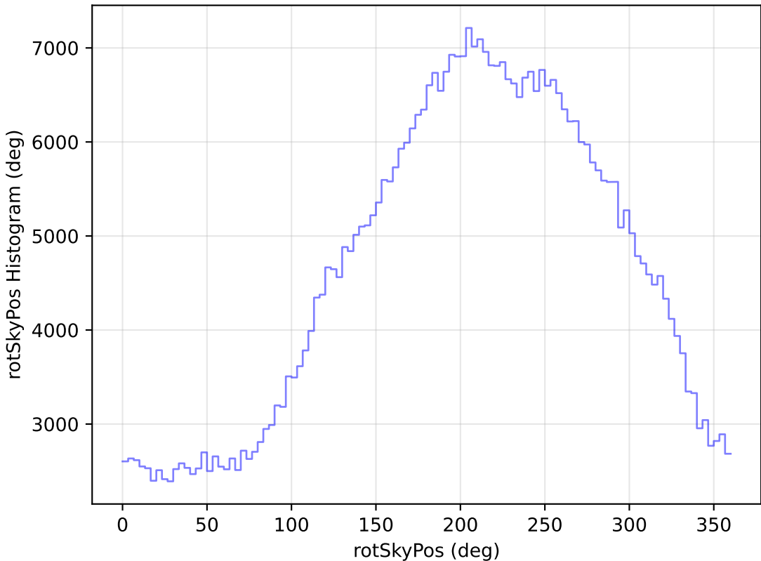
too_elab_r64_d3_griz_v3.4_10yrs All sky i band: rotSkyPos Histogram
