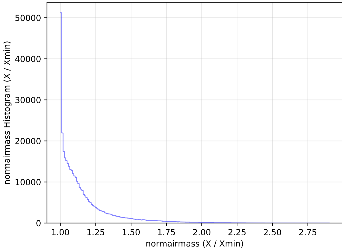
too_elab_r64_d3_griz_v3.4_10yrs WFD y band: normairmass Histogram
