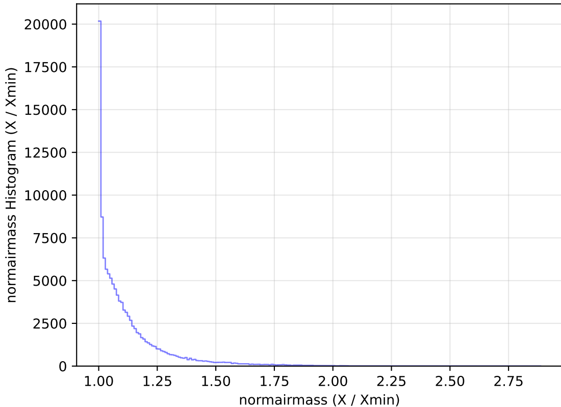
too_elab_r64_d3_griz_v3.4_10yrs WFD u band: normairmass Histogram
