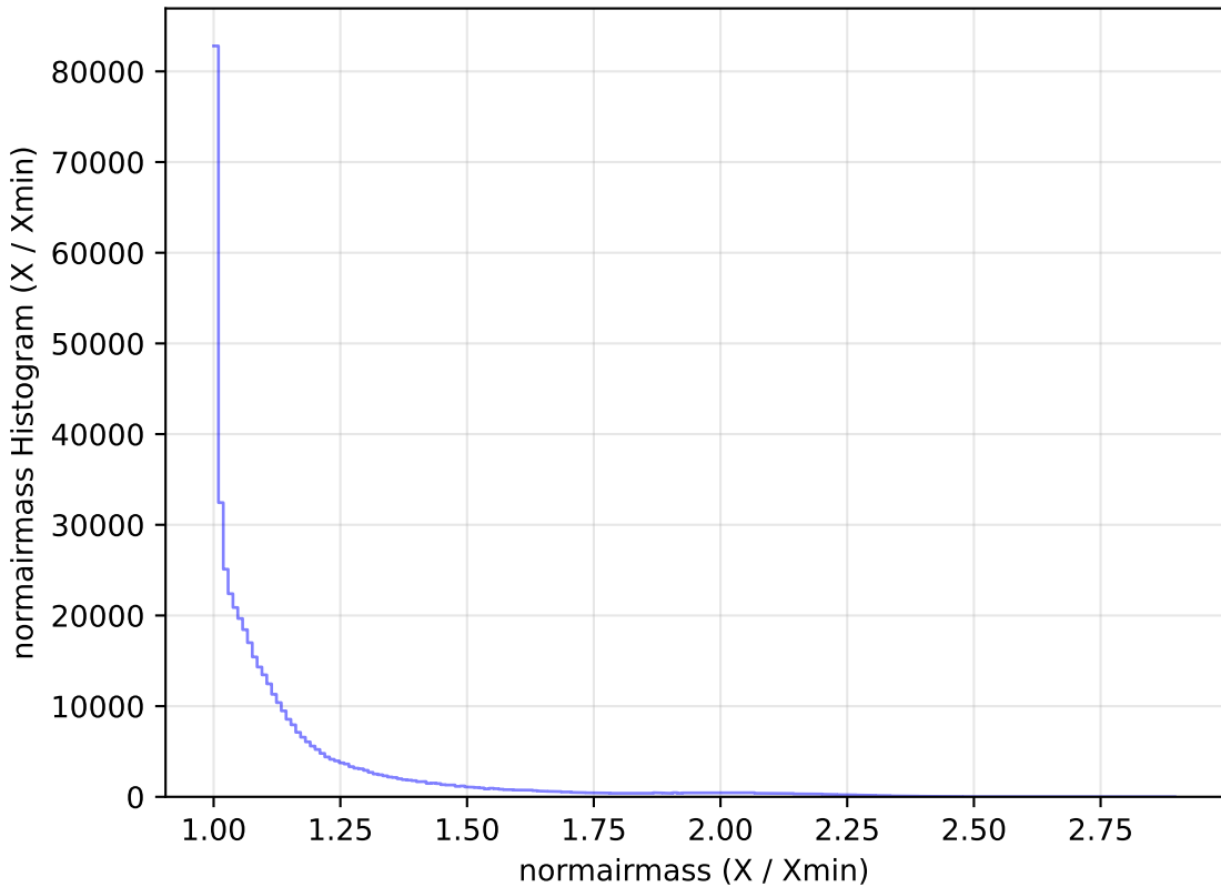
too_elab_r64_d3_griz_v3.4_10yrs WFD r band: normairmass Histogram
