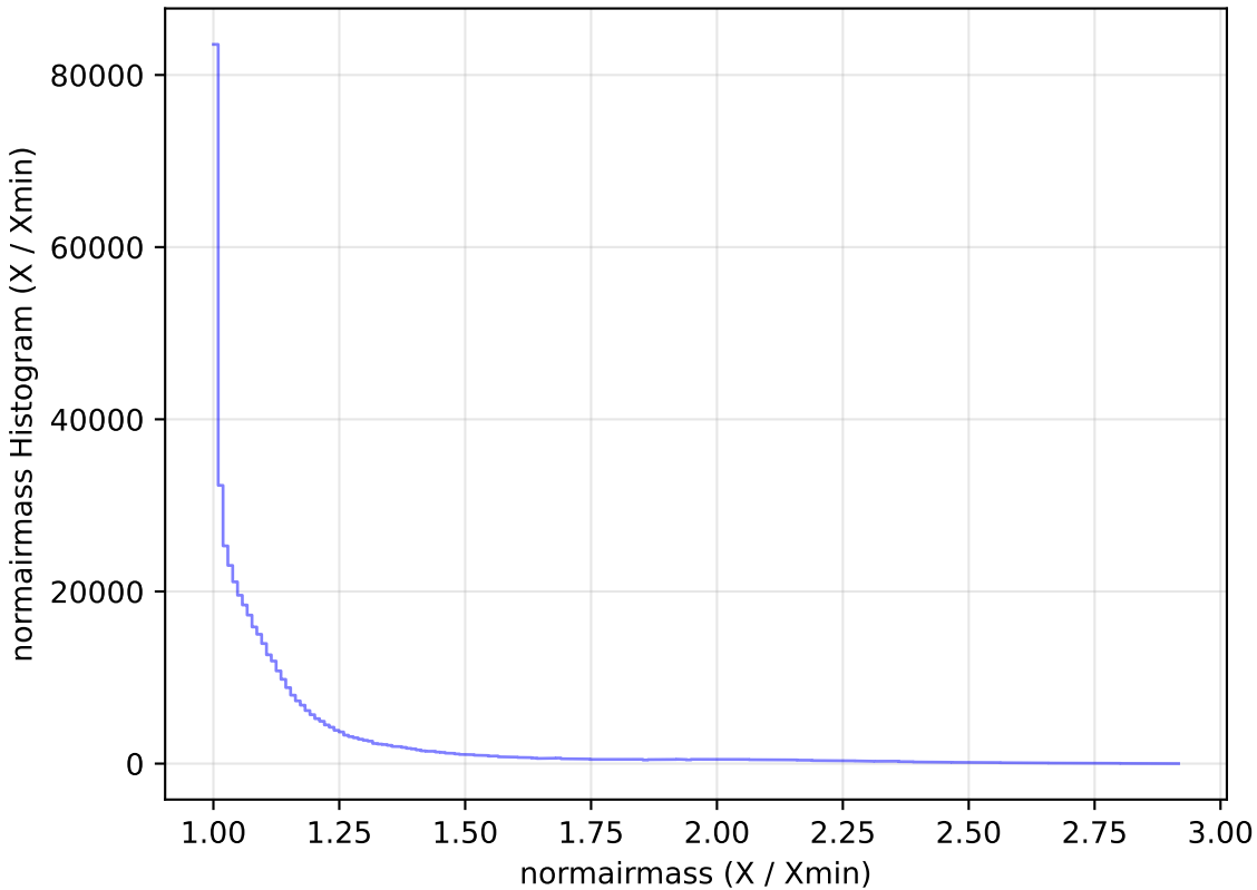
too_elab_r64_d3_griz_v3.4_10yrs WFD i band: normairmass Histogram
