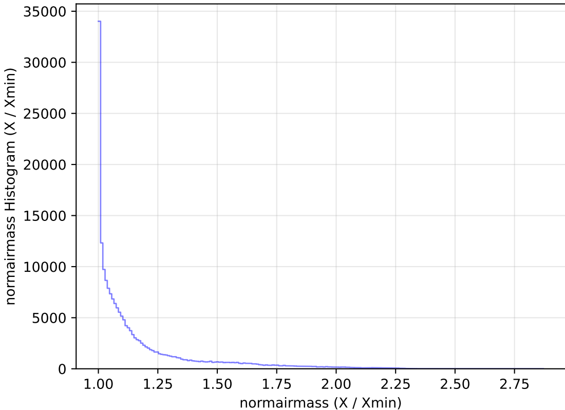
too_elab_r64_d3_griz_v3.4_10yrs WFD g band: normairmass Histogram
