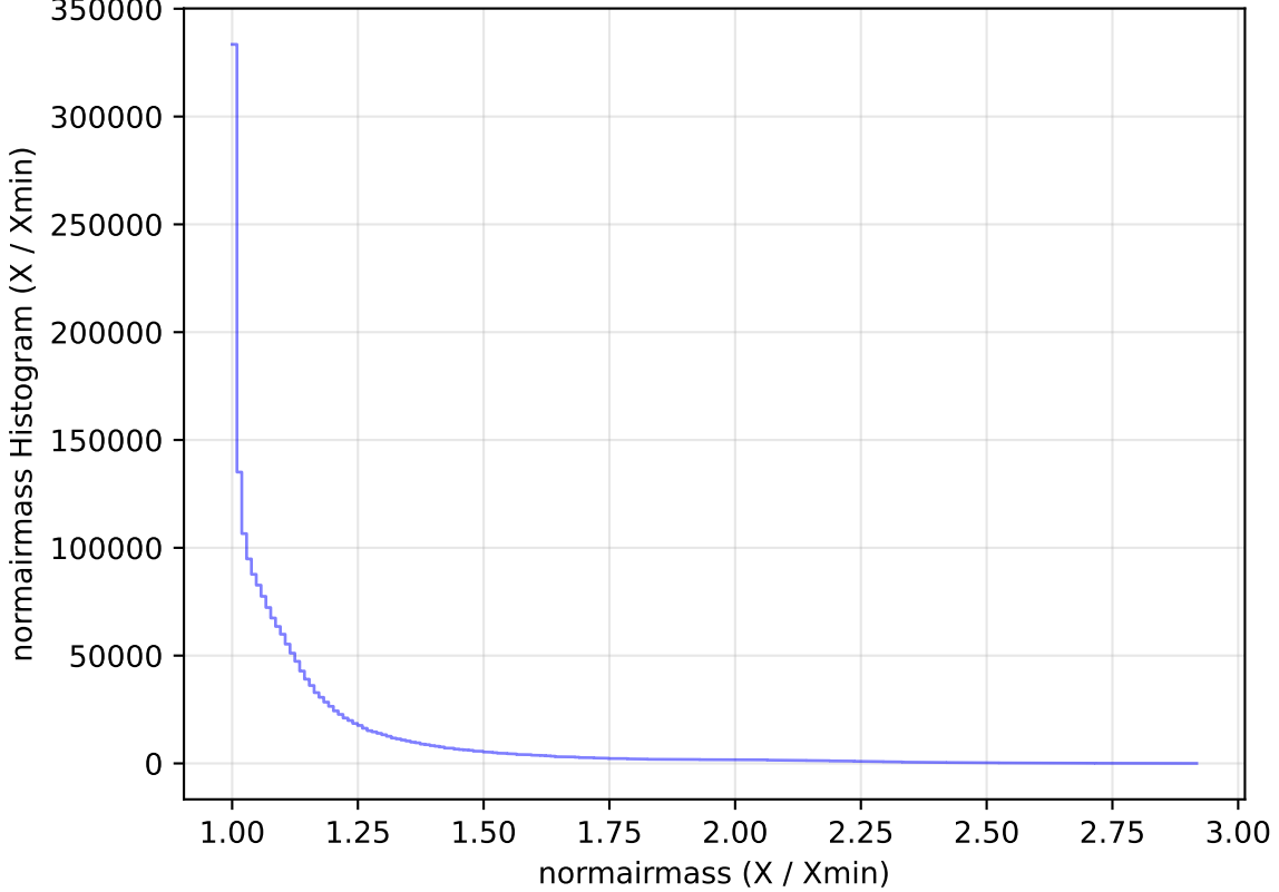
too_elab_r64_d3_griz_v3.4_10yrs WFD all bands: normairmass Histogram
