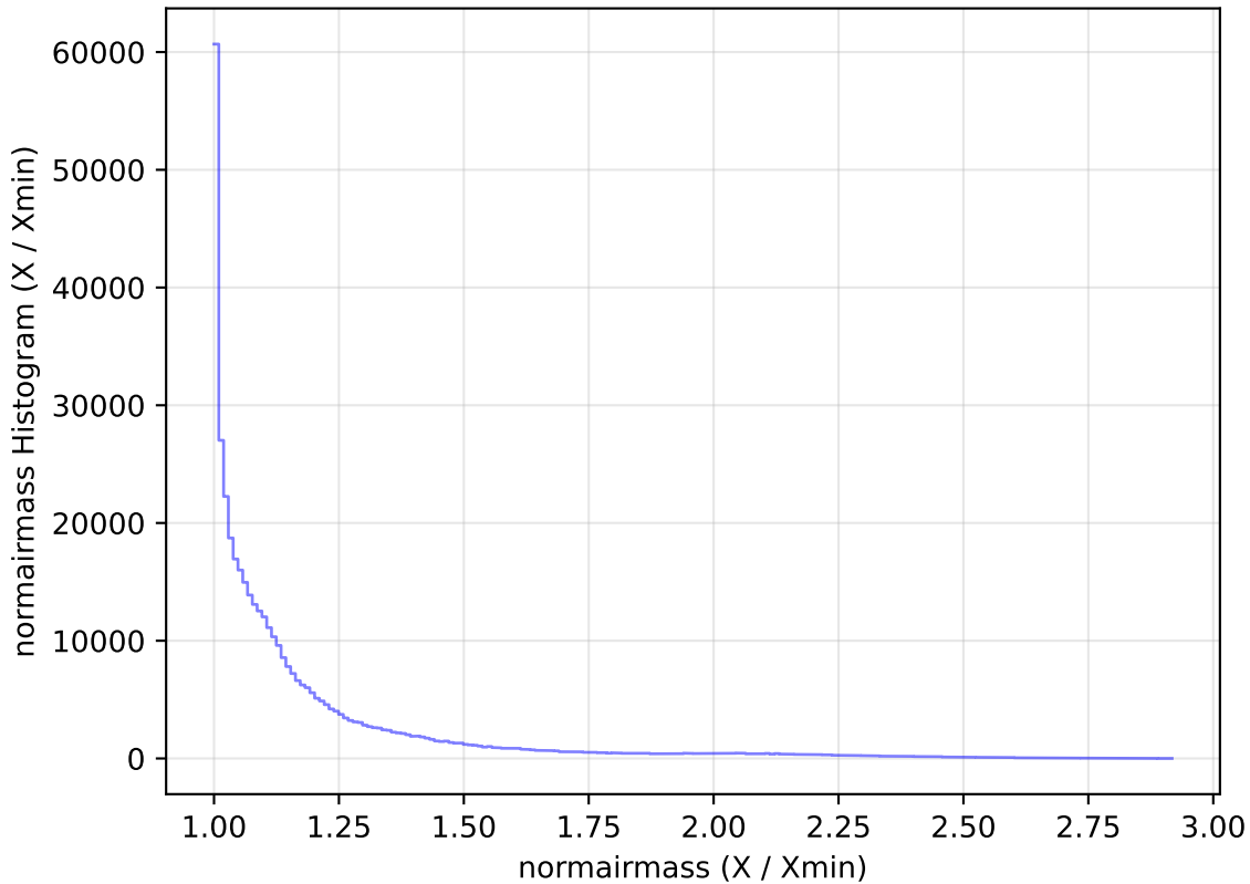
too_elab_r64_d3_griz_v3.4_10yrs All sky z band: normairmass Histogram
