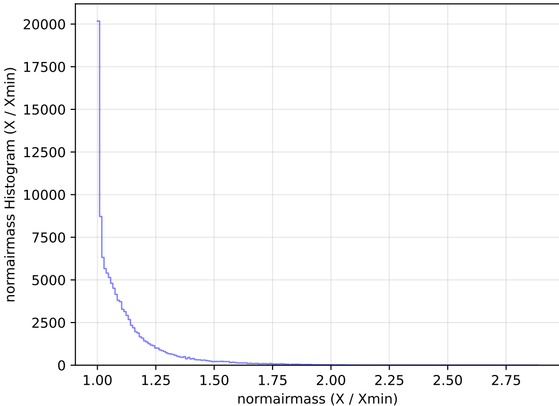
too_elab_r64_d3_griz_v3.4_10yrs All sky u band: normairmass Histogram
