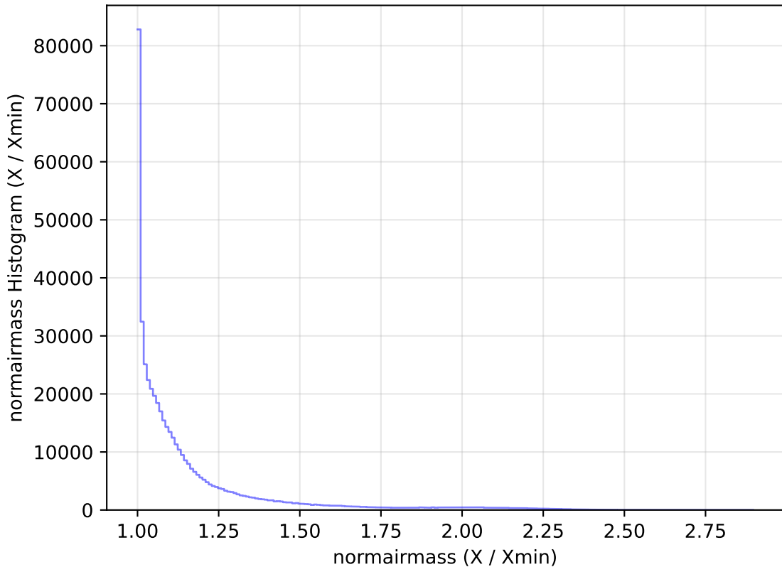
too_elab_r64_d3_griz_v3.4_10yrs All sky r band: normairmass Histogram
