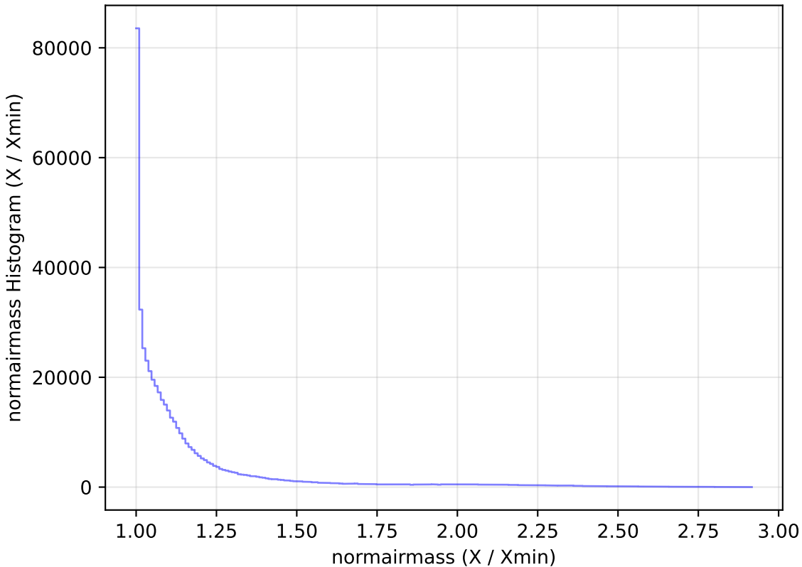
too_elab_r64_d3_griz_v3.4_10yrs All sky i band: normairmass Histogram
