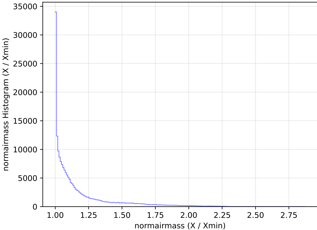
too_elab_r64_d3_griz_v3.4_10yrs All sky g band: normairmass Histogram
