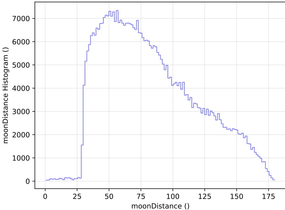
too_elab_r64_d3_griz_v3.4_10yrs WFD z band: moonDistance Histogram
