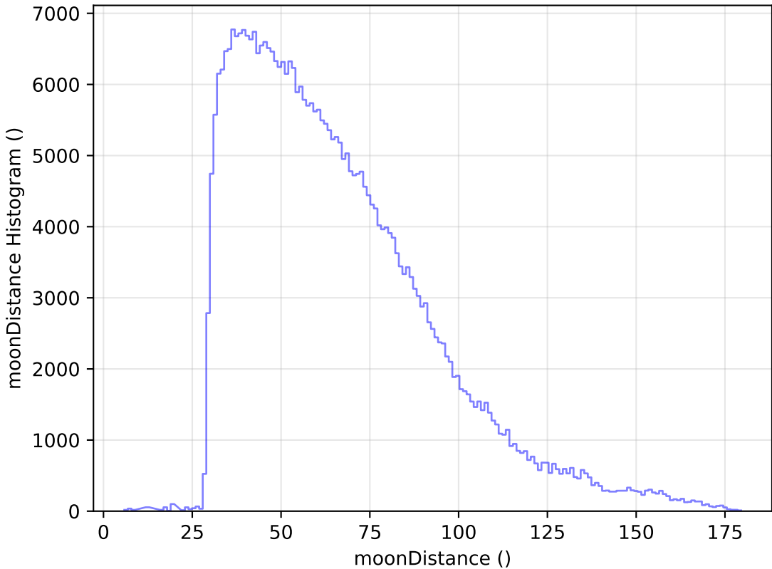
too_elab_r64_d3_griz_v3.4_10yrs WFD y band: moonDistance Histogram
