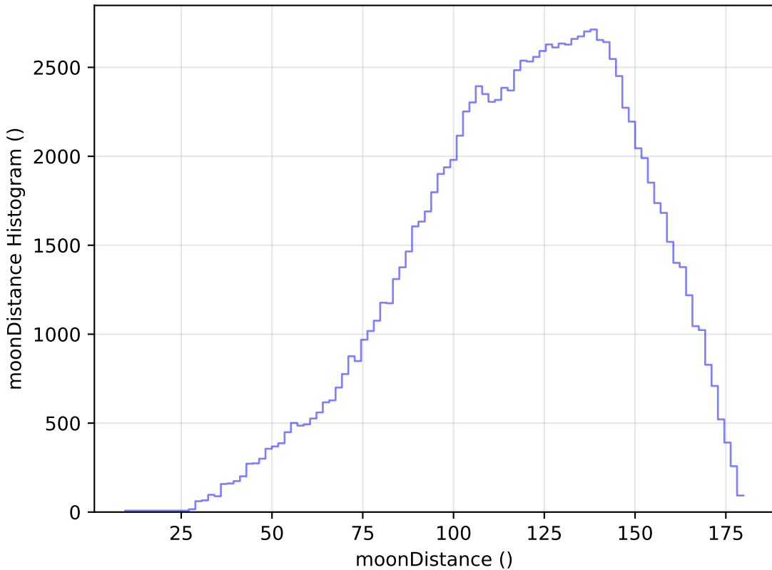
too_elab_r64_d3_griz_v3.4_10yrs WFD u band: moonDistance Histogram
