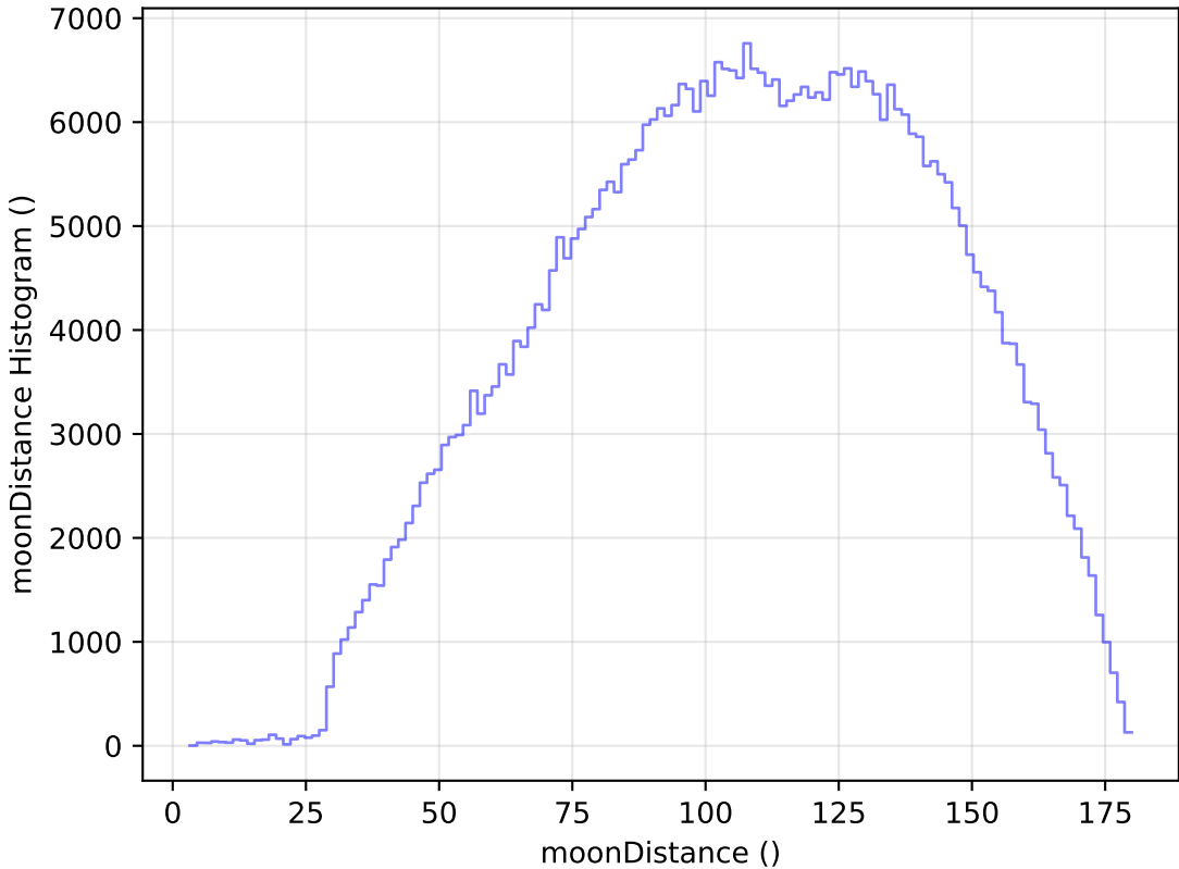
too_elab_r64_d3_griz_v3.4_10yrs WFD r band: moonDistance Histogram
