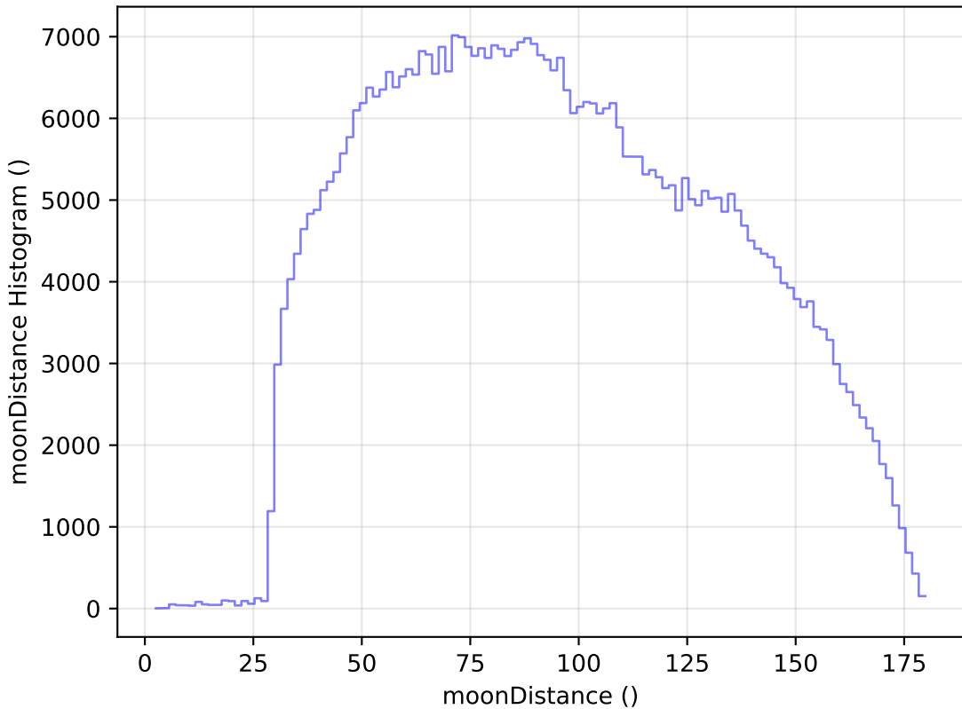
too_elab_r64_d3_griz_v3.4_10yrs WFD i band: moonDistance Histogram
