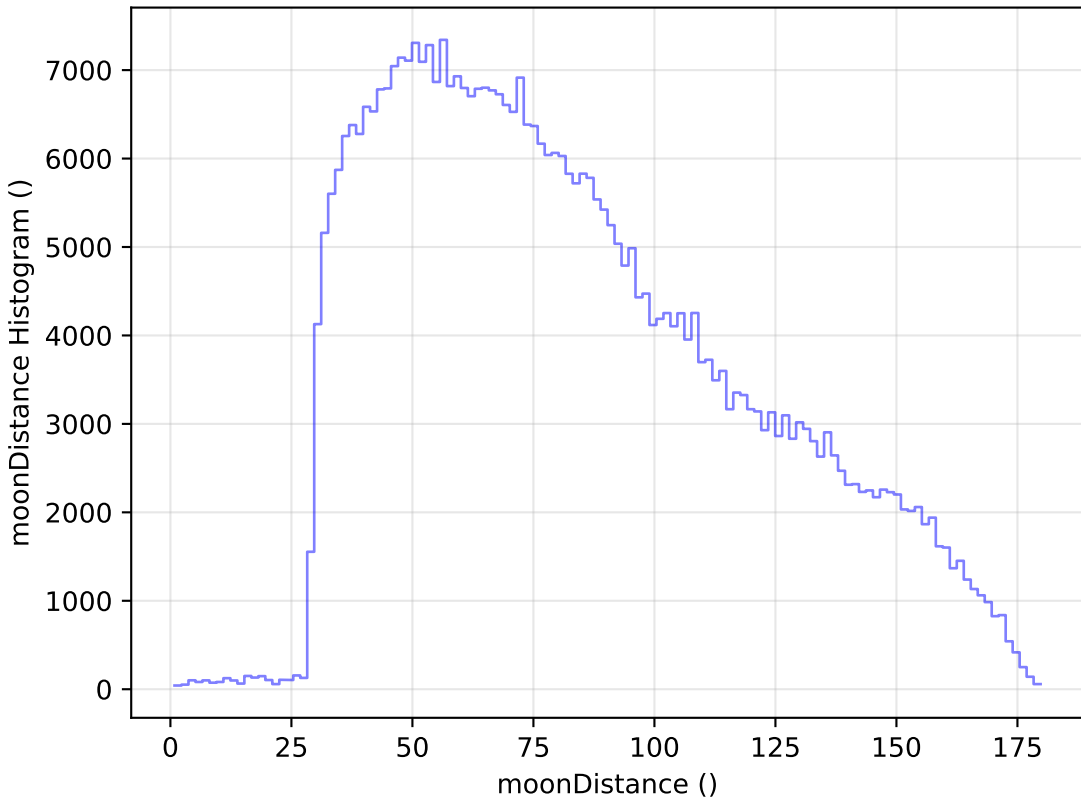
too_elab_r64_d3_griz_v3.4_10yrs All sky z band: moonDistance Histogram
